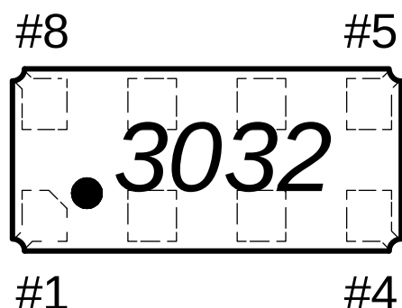
TS-3032-C7 Package: (top view)
